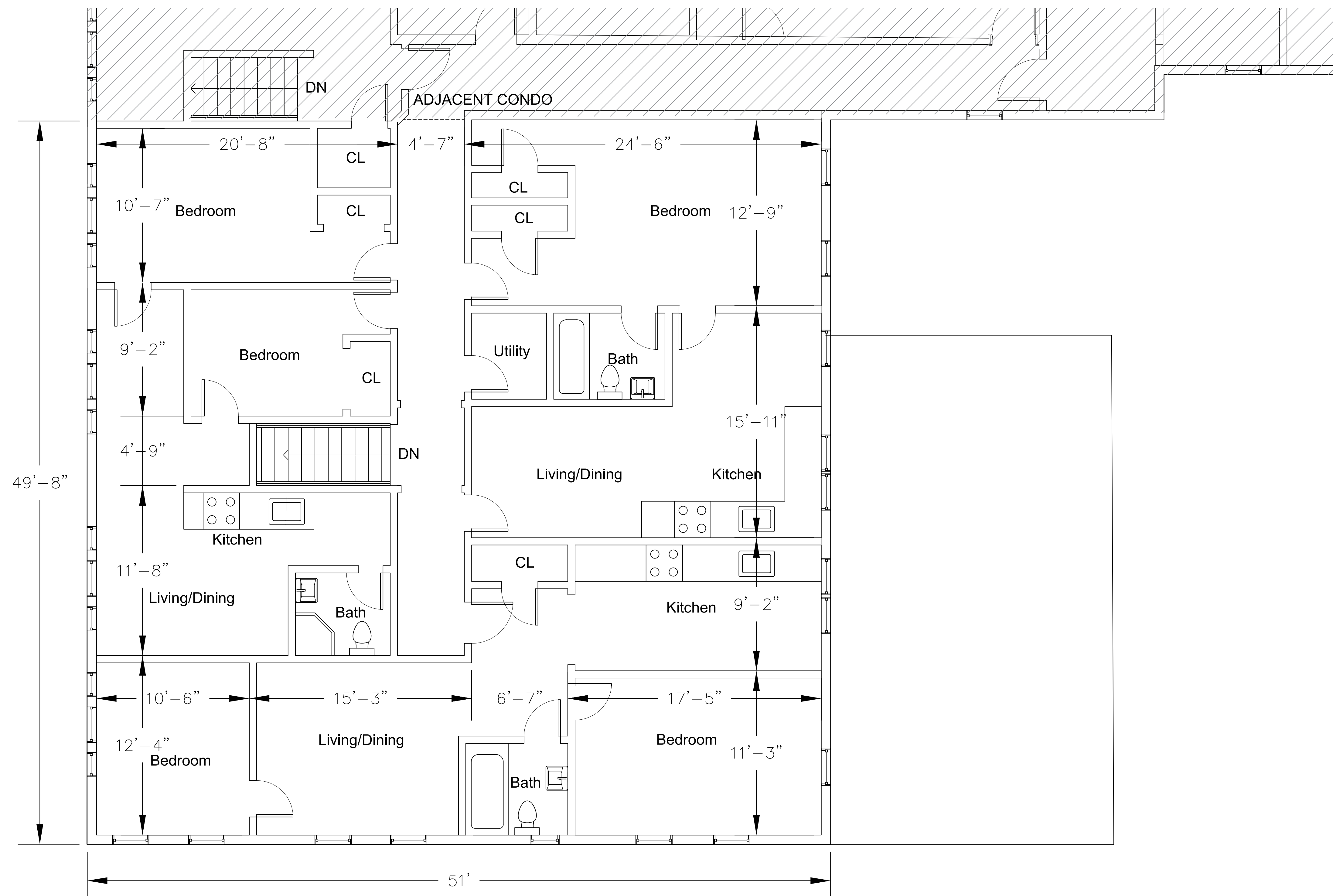
1 FLOOR PLAN - LEVEL 2 1/4" = 1'-0"
