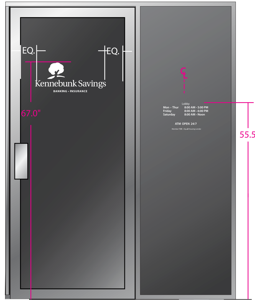
ELEVATION - TYPICAL SCALE: 3/4"=1'-0"
